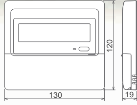
Unit: mm
