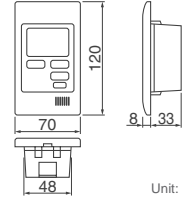
Unit: mm
